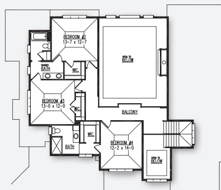
Second Floor 1,080 Sq. Ft.
