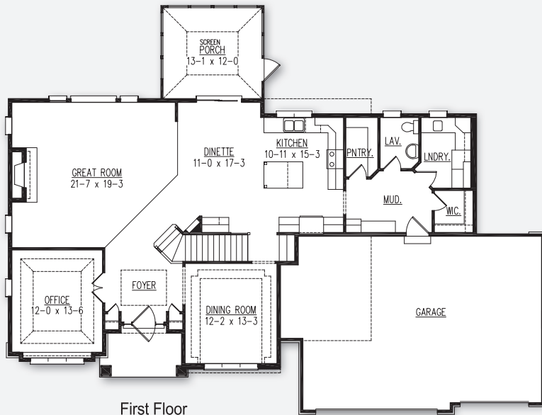
First Floor 1,638 Sq. Ft.
