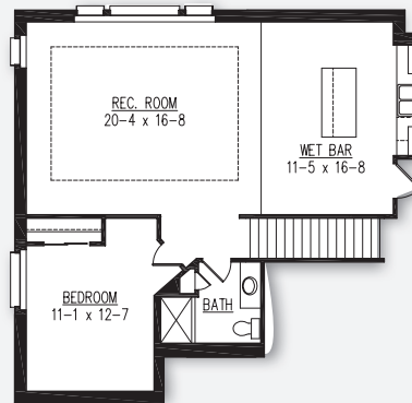
Finished Lower Level Adds 823 Sq. Ft.
