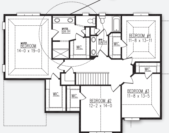
SECOND FLOOR 1,422 SQ. FT.
