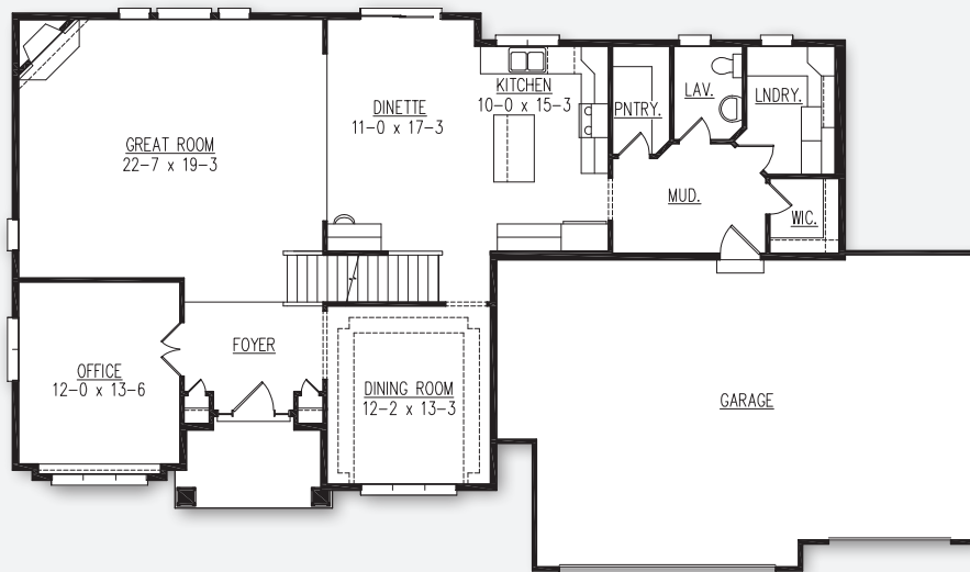
FIRST FLOOR 1,629 SQ. FT.
