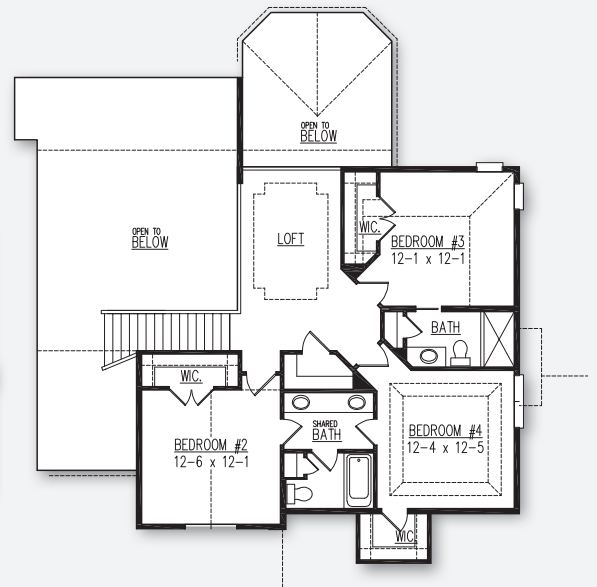
SECOND FLOOR 974 SQ. FT.
