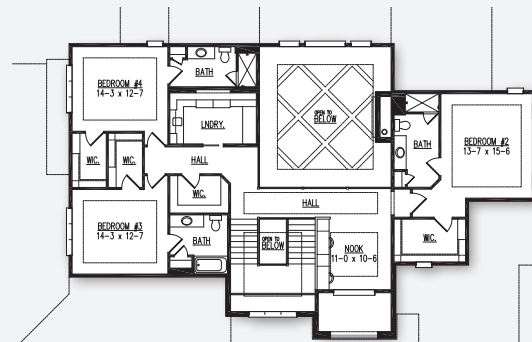
Second Floor 1,630 Sq. Ft.
