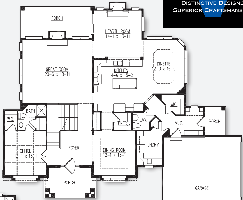
First Floor 2,145 Sq. Ft.
