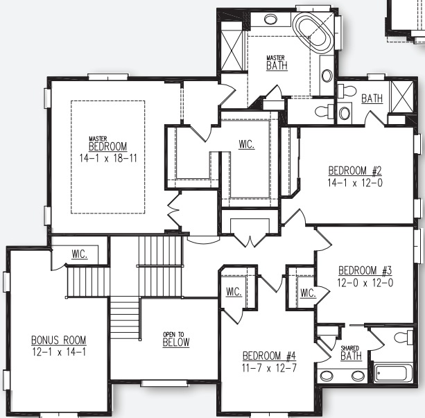
Second Floor 1,857 Sq. Ft.
