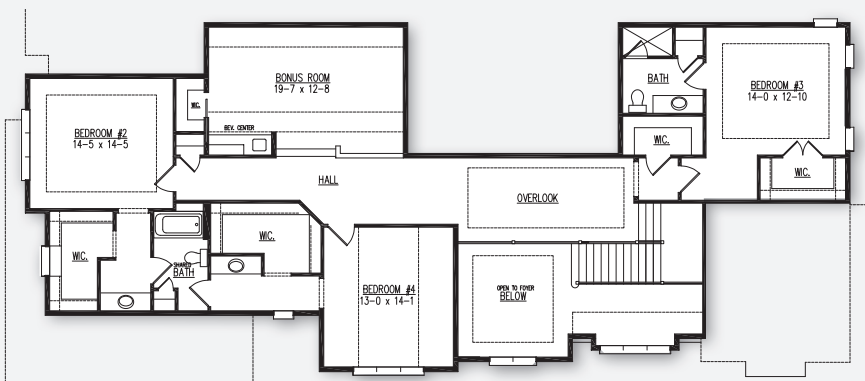
Second Floor 1,760 Sq. Ft.
